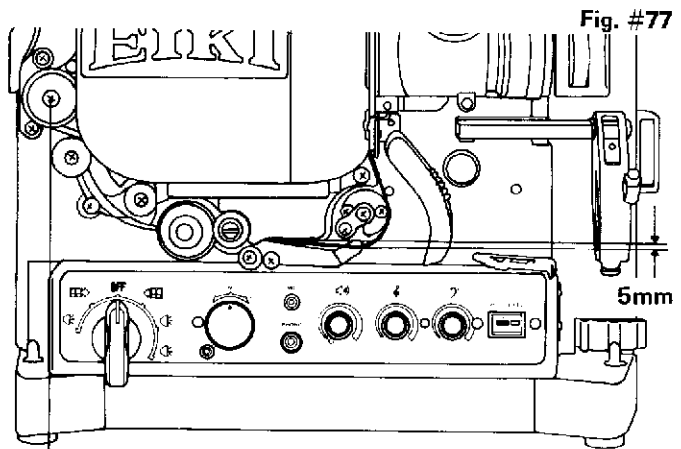
#2 SPROCKET COVER SCREW
