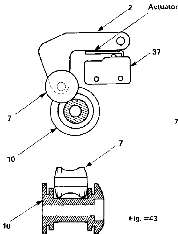
No film in the threading path Sensor micro switch (37) ON
